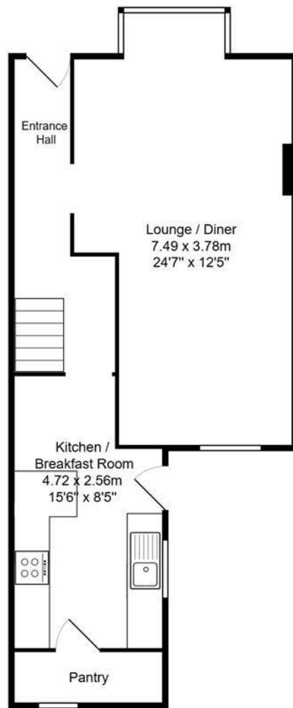
Ground Floor Area: 45.0 m 2 ... 484 ft 2
