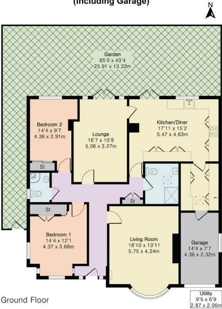
Approximate Gross Internal Area 1384 sq ft - 129 sq m (Including Garage)
