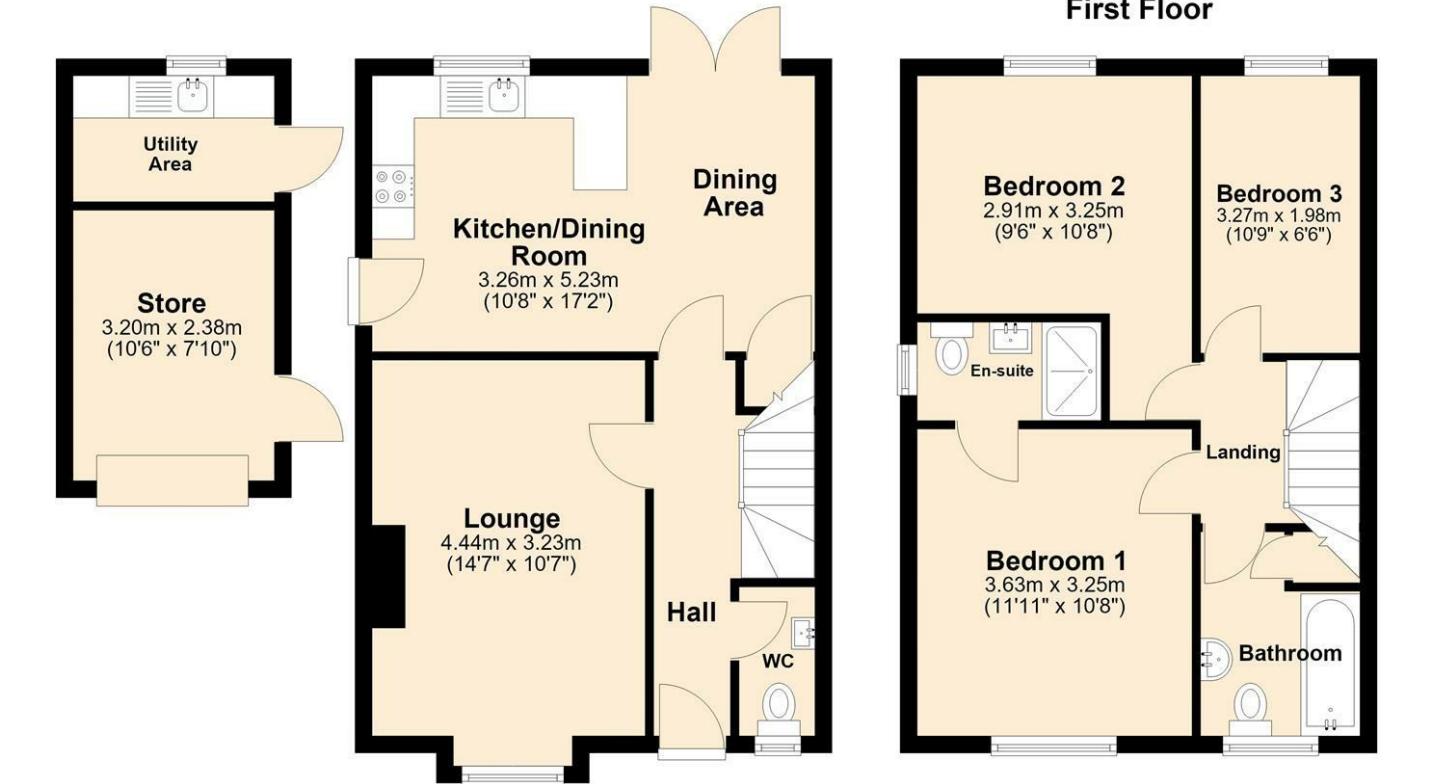
Ground Floor
