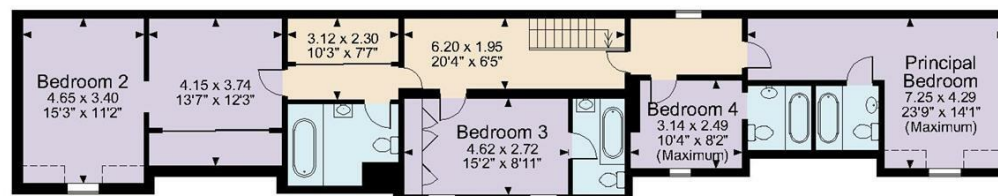
First Floor
