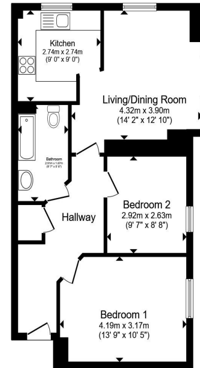
2nd Floor
