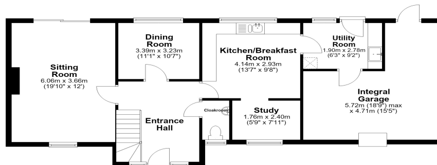
Ground Floor Approx. 82.0 sq. metres (882.4 sq. feet)
