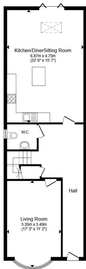
Ground Floor
