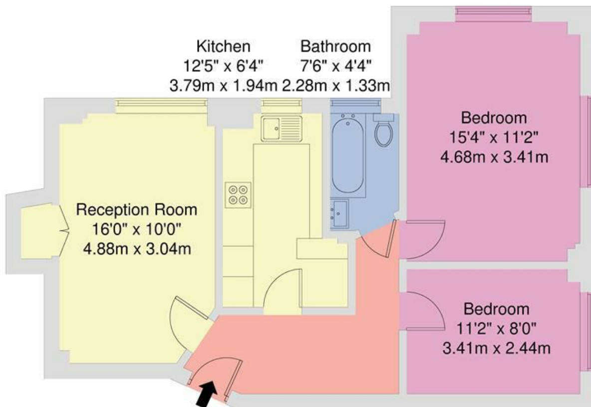
GROUND FLOOR
