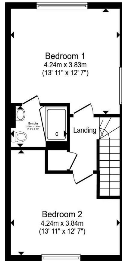
Second Floor
