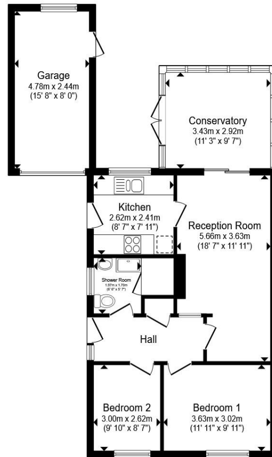
Floor Plan
