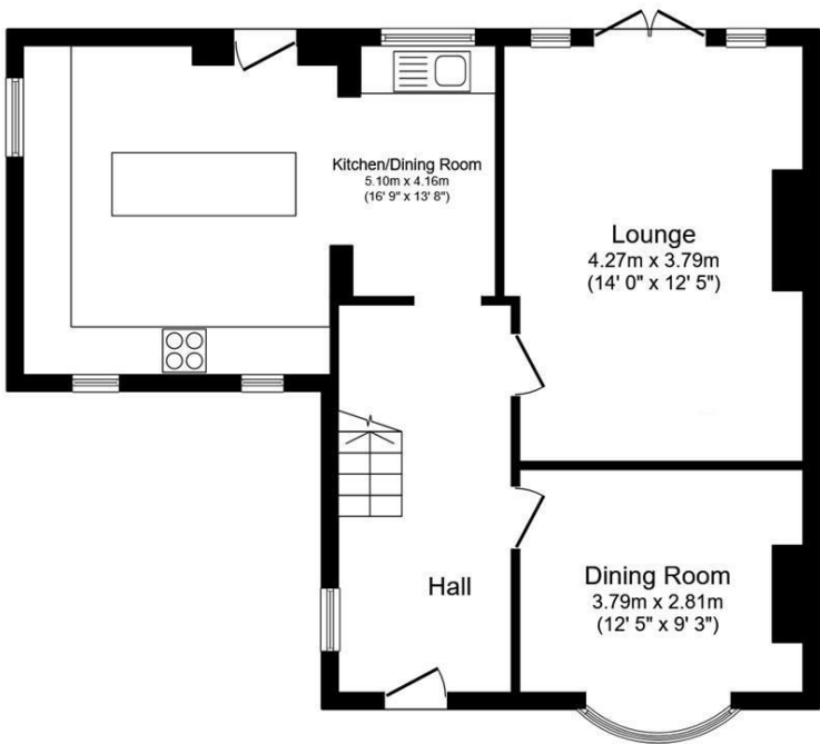
Ground Floor Floor area 64.8 sq.m. (697 sq.ft.)
