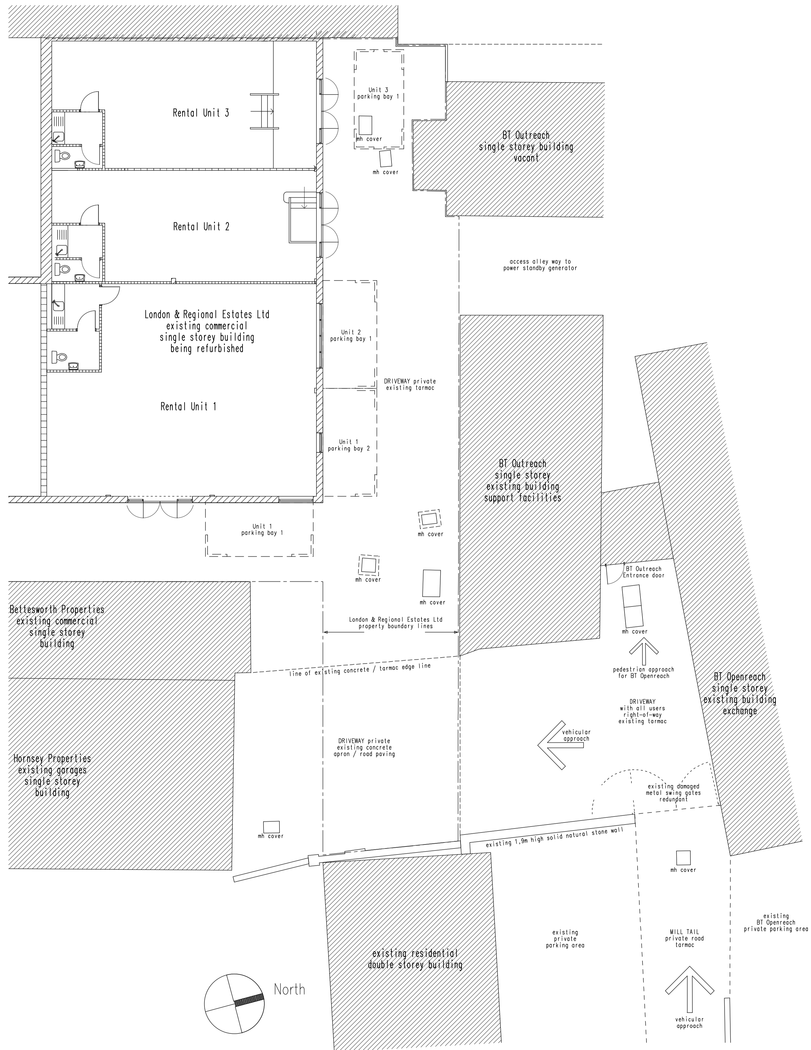
SITE LAYOUT PLAN scale 1:200
