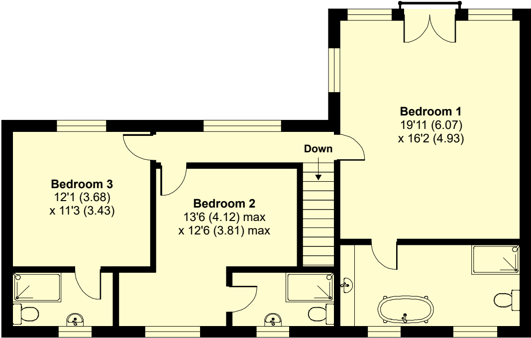
FIRST FLOOR
