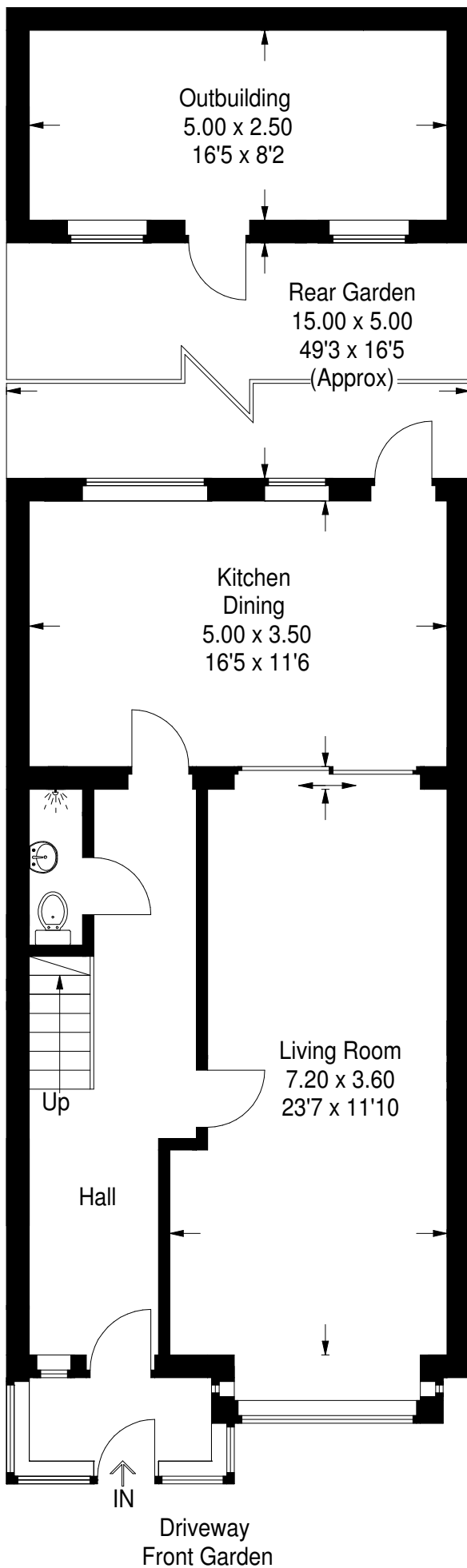
Ground Floor
