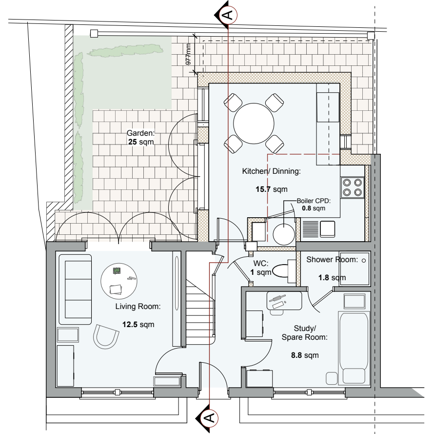
PROPOSED Groun Floor PLAN SCALE - 1:100 AT A3
