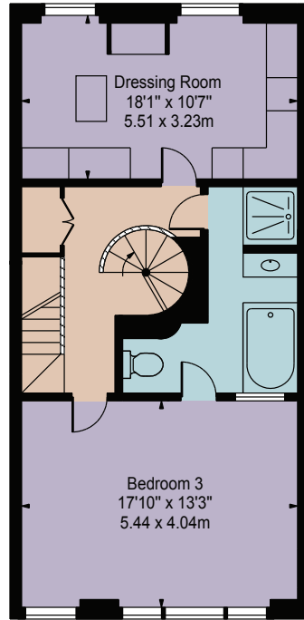
Third Floor
