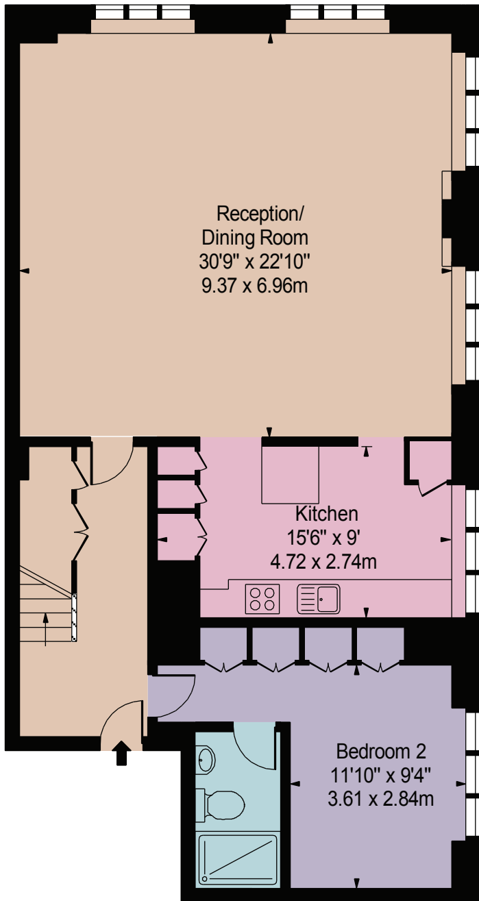
Third Floor
