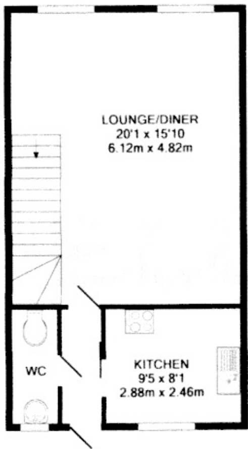
GROUND FLOOR APPROX. FLOOR AREA 445 SQ. FT. (41.4 SQ. M.)
