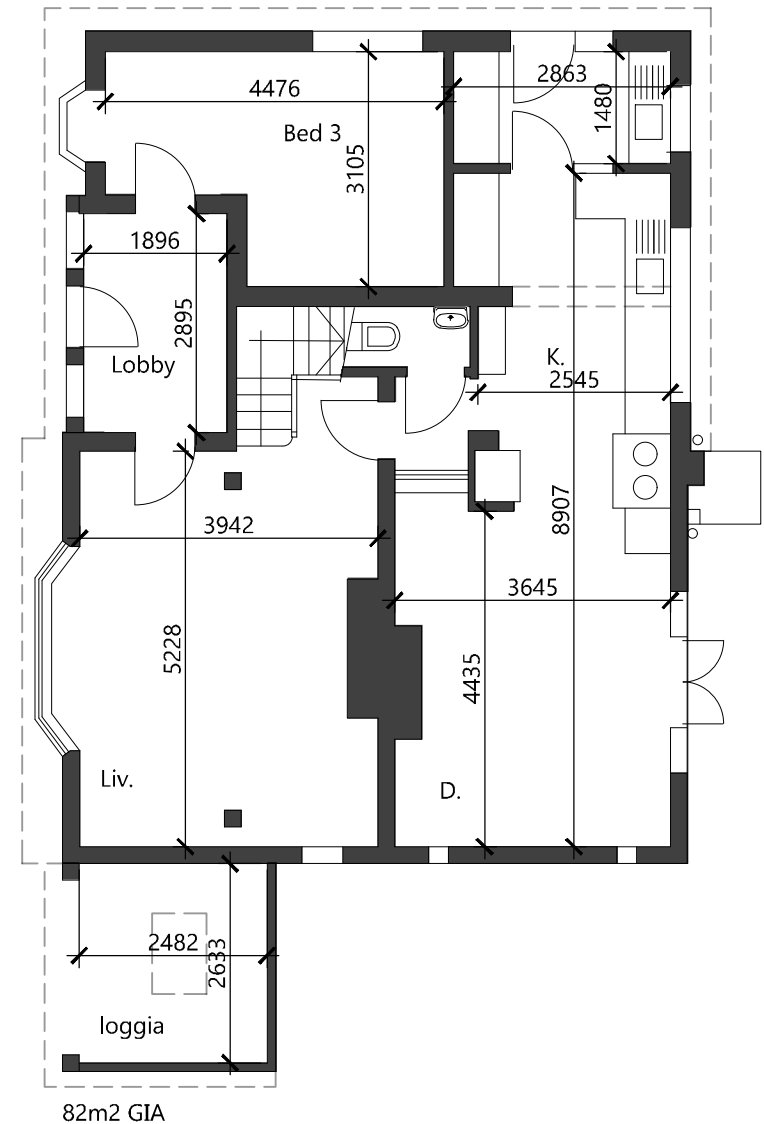
Ground floor 1:100
