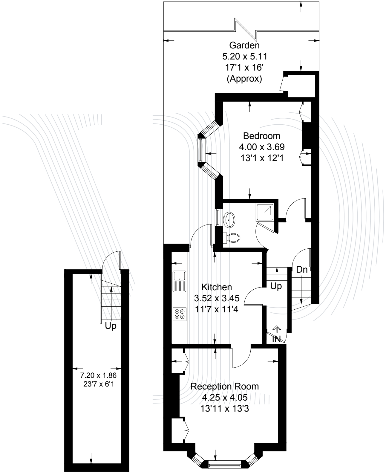
Basement Floor 143 sq ft / 13.3 sq m
