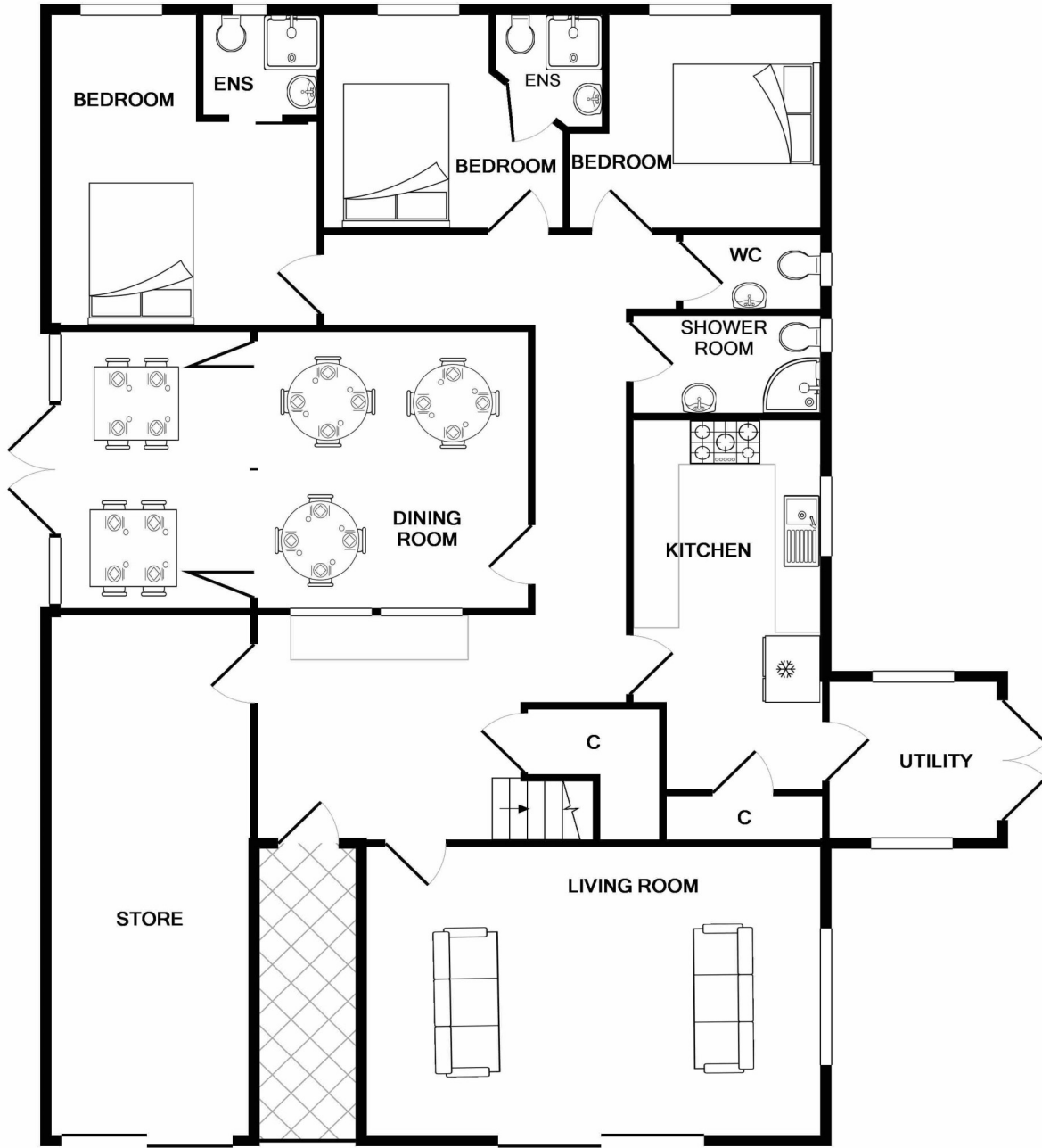
GROUND FLOOR
