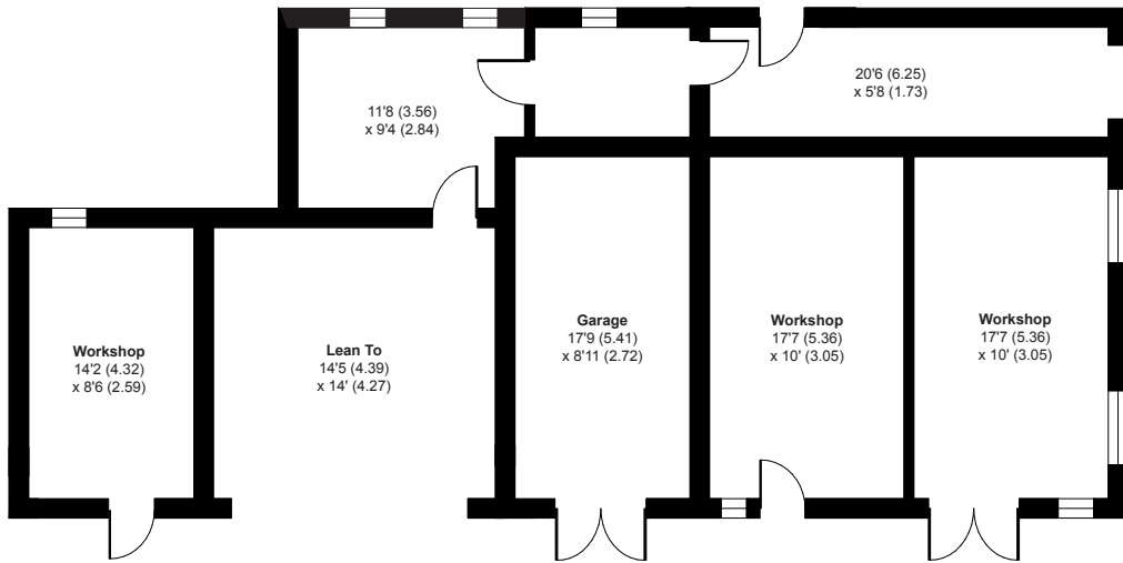
OUTBUILDING 1
